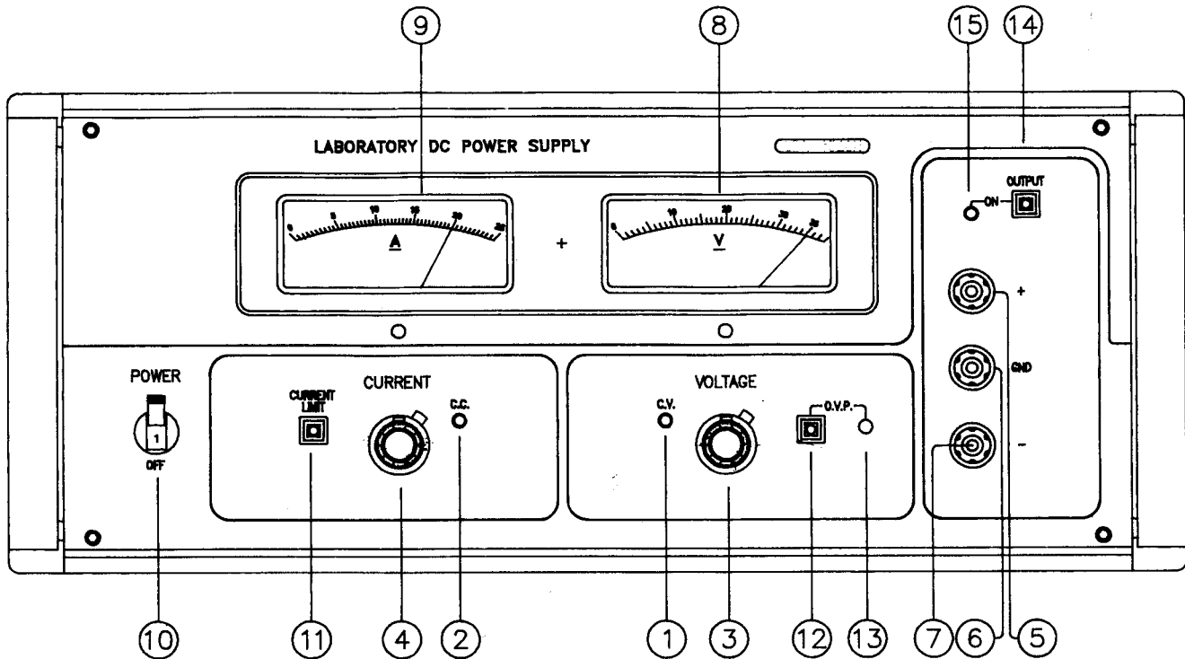
Fig. 4-2 Front Panel (Analog Type)
