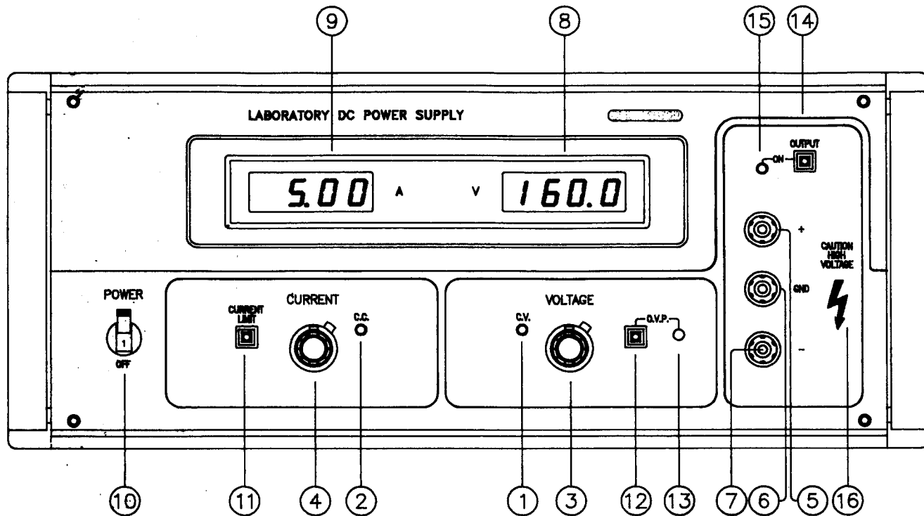
Fig. 4-1 Front Panel (Digital Type)
