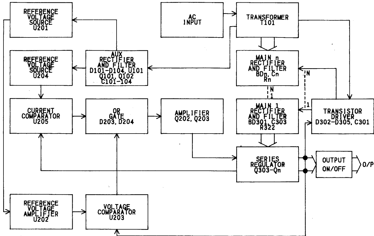
Fig. 2 Block Diagram (More Than 100V)
